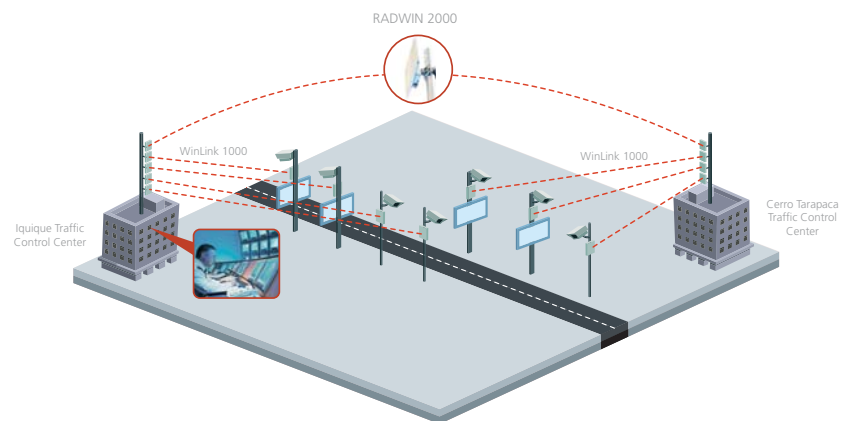
Video surveillance transmission along Chile’s A-16 highway
